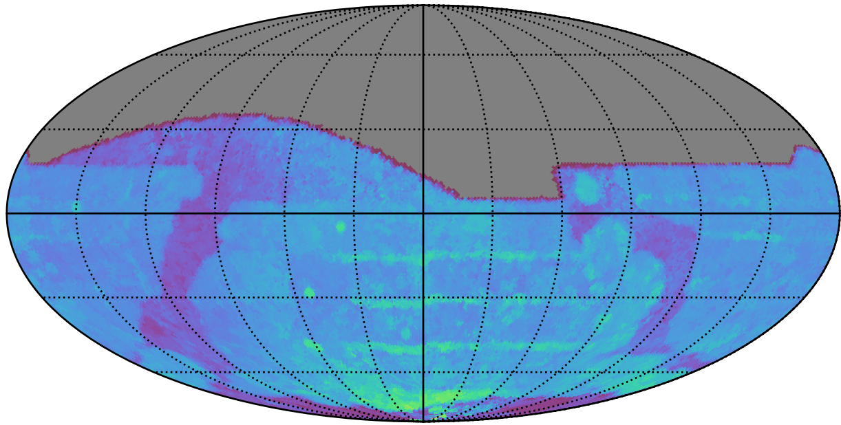
ddf_acor_sf10_lsf30_lsr10_v3.4_10yrs All sky i band: 80thPercentile Season Length
