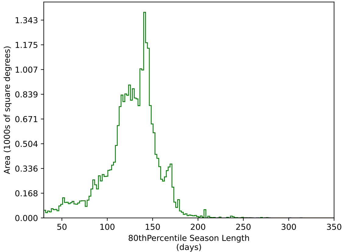
ddf_acor_sf10_lsf30_lsr10_v3.4_10yrs All sky g band: 80thPercentile Season Length
