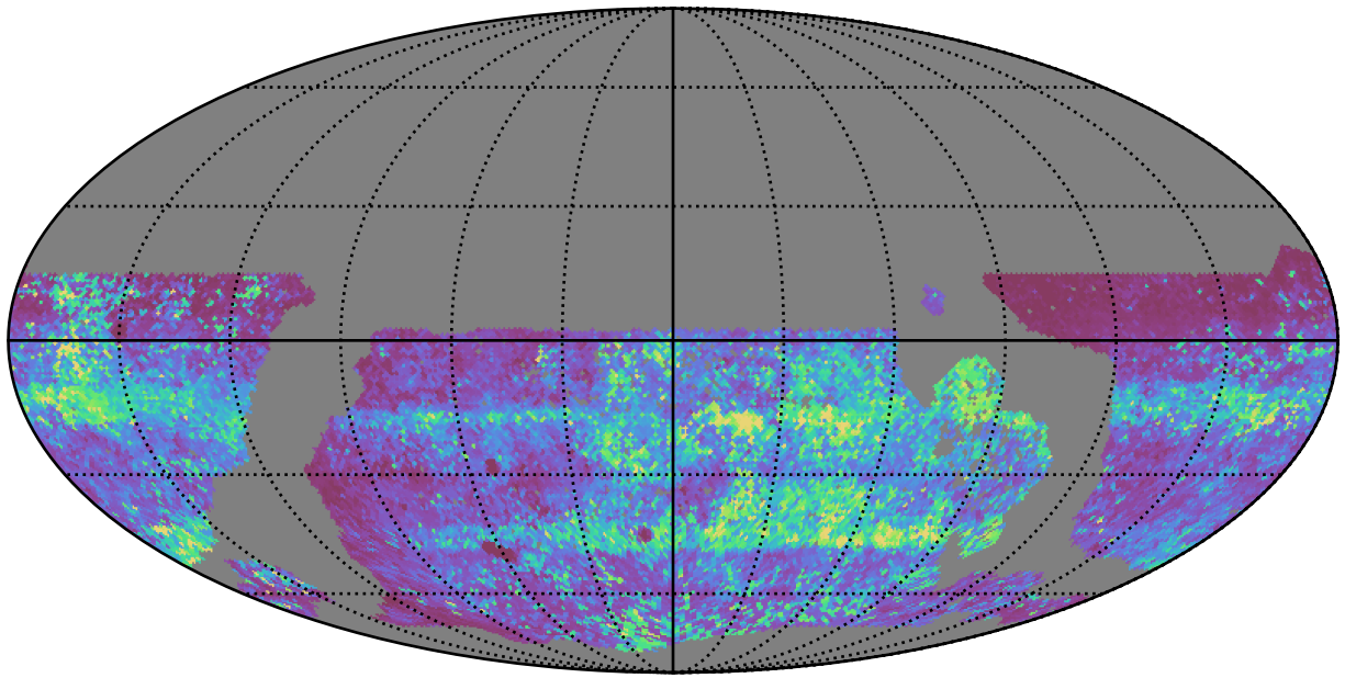
ddf_acor_sf10_lsf30_lsr10_v3.4_10yrs WFD zy bands: 75th Percentile Intranight Timespan
