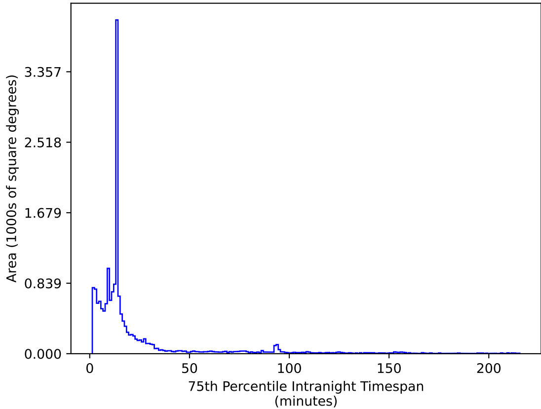
ddf_acor_sf10_lsf30_lsr10_v3.4_10yrs WFD z band: 75th Percentile Intranight Timespan
