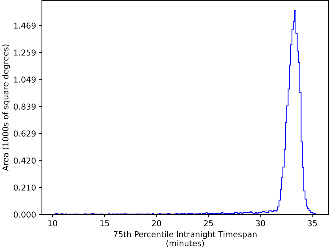
ddf_acor_sf10_lsf30_lsr10_v3.4_10yrs WFD ug bands: 75th Percentile Intranight Timespan
