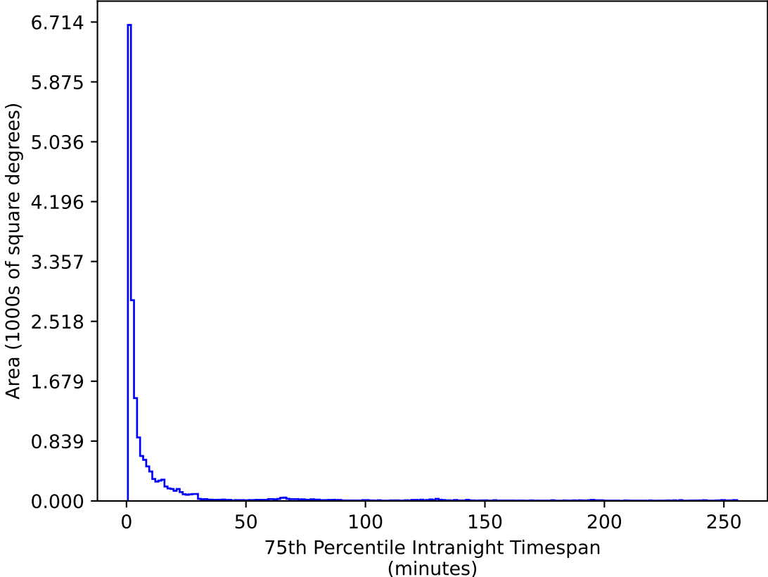
ddf_acor_sf10_lsf30_lsr10_v3.4_10yrs WFD u band: 75th Percentile Intranight Timespan
