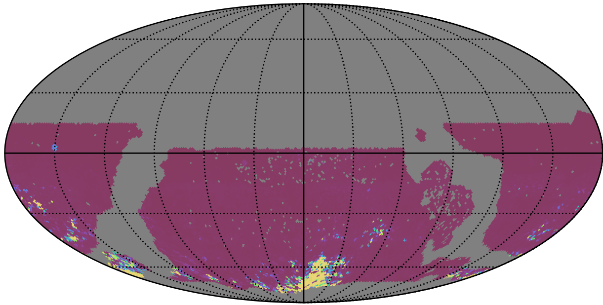
ddf_acor_sf10_lsf30_lsr10_v3.4_10yrs WFD ri bands: 75th Percentile Intranight Timespan
