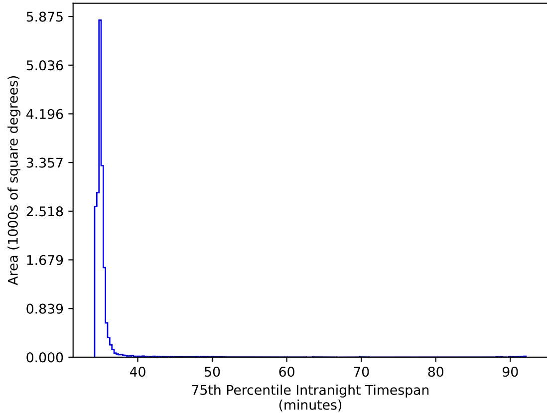
ddf_acor_sf10_lsf30_lsr10_v3.4_10yrs WFD ri bands: 75th Percentile Intranight Timespan
