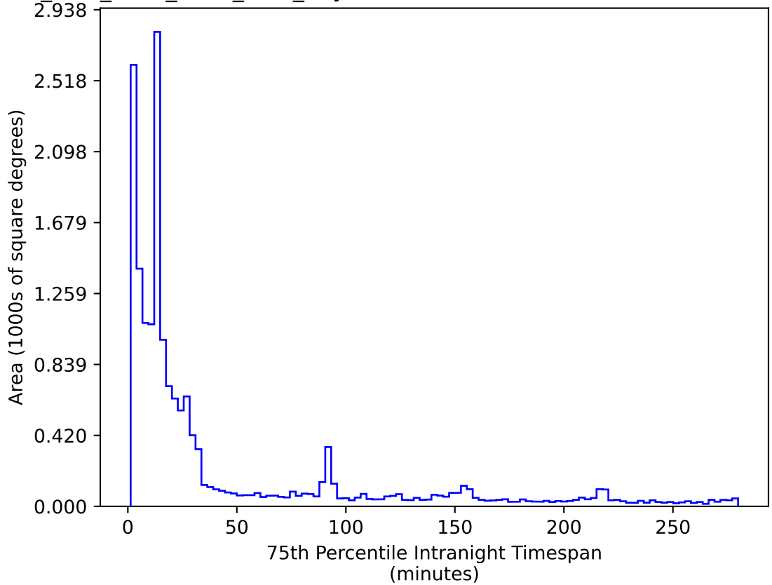
ddf_acor_sf10_ls30_lsr10_v3.4_10yrs WFD r band: 75th Percentile Intranight Timespan
