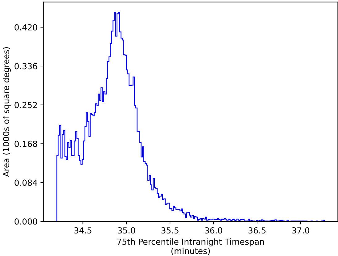
ddf_acor_sf10_ls30_lsr10_v3.4_10yrs WFD iz bands: 75th Percentile Intranight Timespan
