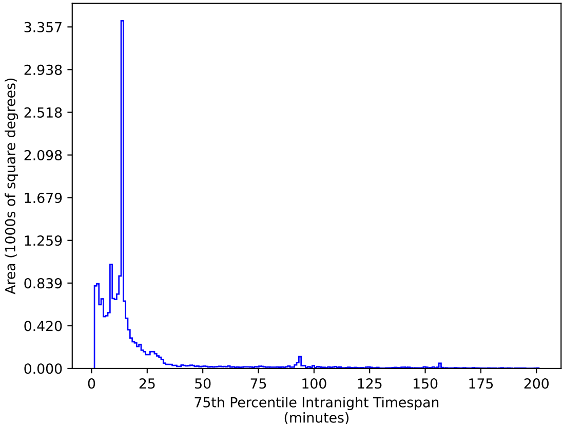
ddf_acor_sf10_lsf30_lsr10_v3.4_10yrs WFD i band: 75th Percentile Intranight Timespan
