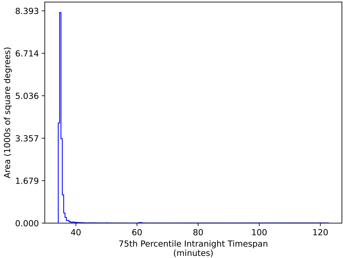
ddf_acor_sf10_lsf30_lsr10_v3.4_10yrs WFD gr bands: 75th Percentile Intranight Timespan
