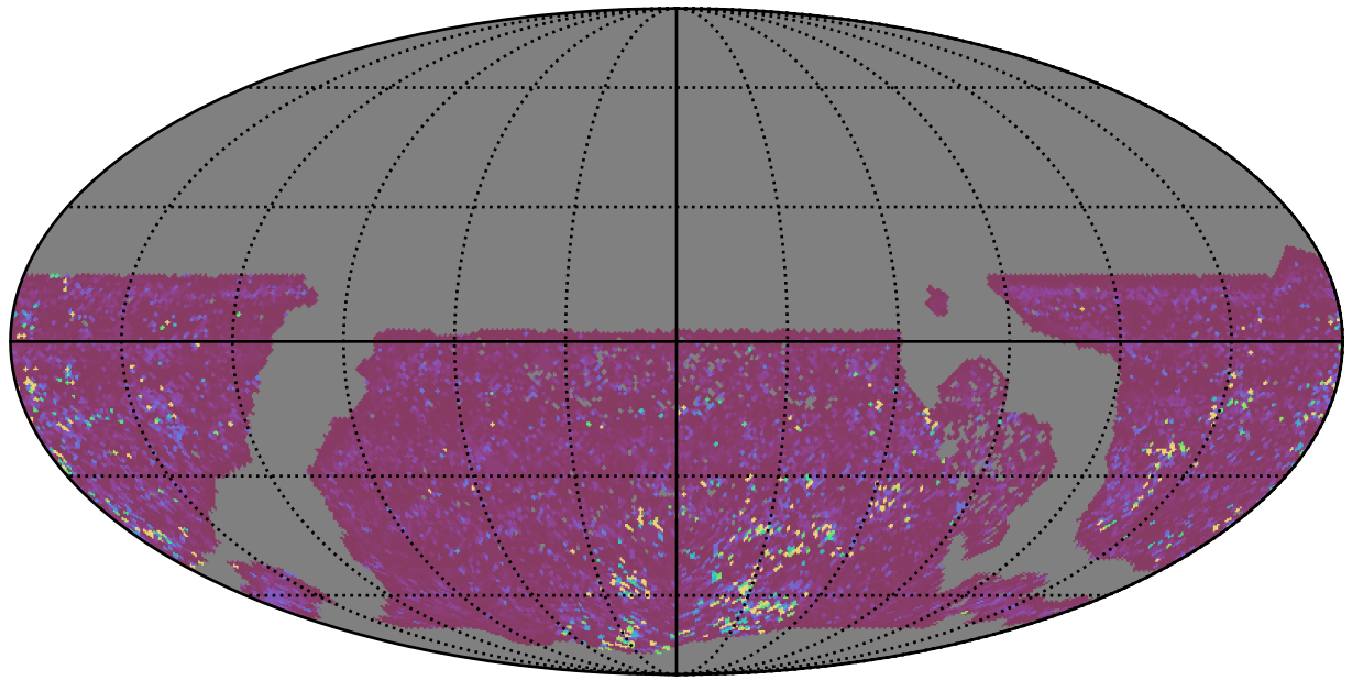
ddf_acor_sf10_lsf30_lsr10_v3.4_10yrs WFD g band: 75th Percentile Intranight Timespan
