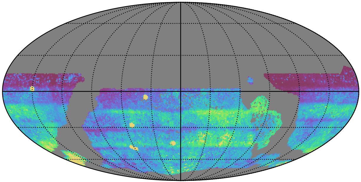
ddf_acor_sf10_lsf30_lsr10_v3.4_10yrs WFD all bands: 75th Percentile Intranight Timespan
