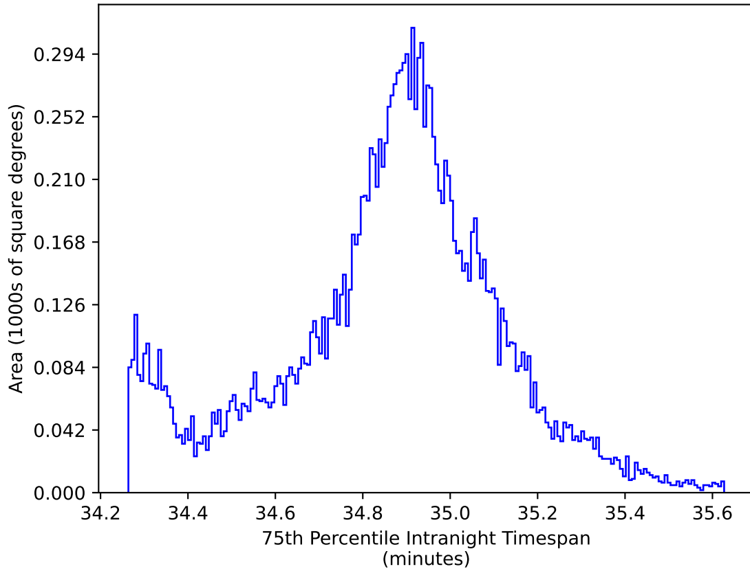
ddf_acor_sf10_ls30_lsr10_v3.4_10yrs WFD all bands: 75th Percentile Intranight Timespan
