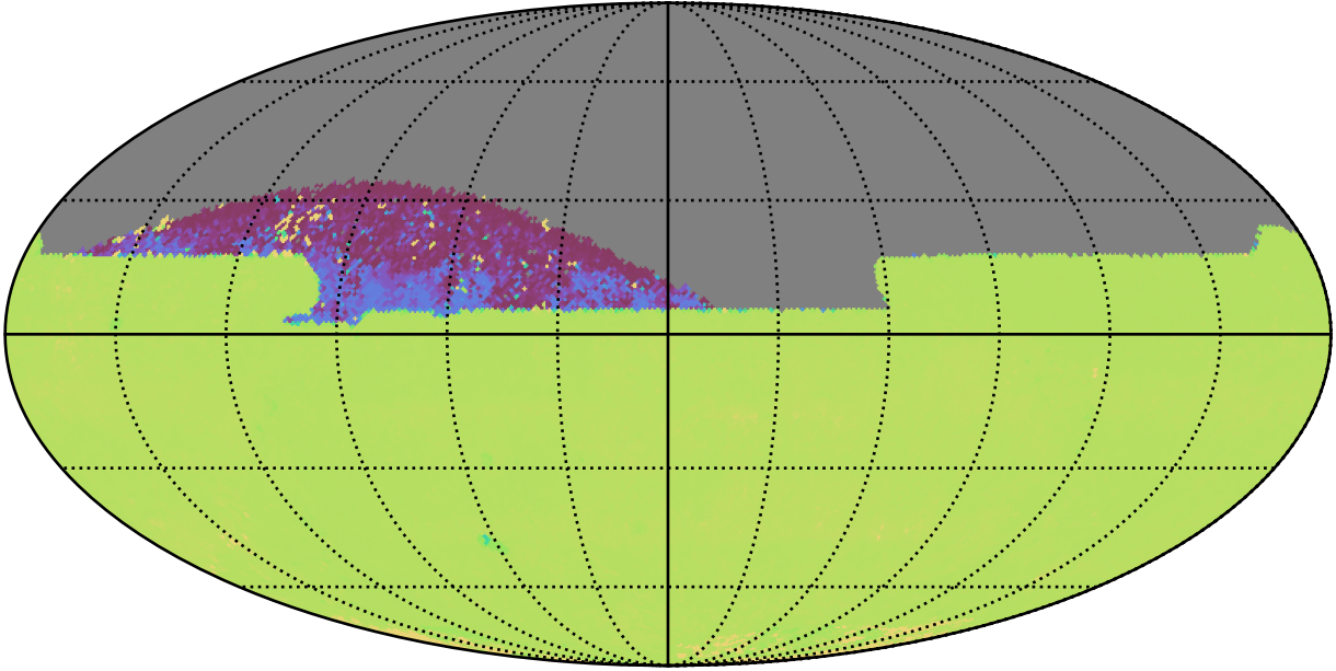
ddf_acor_sf10_lsf30_lsr10_v3.4_10yrs All sky zy bands: 75th Percentile Intranight Timespan
