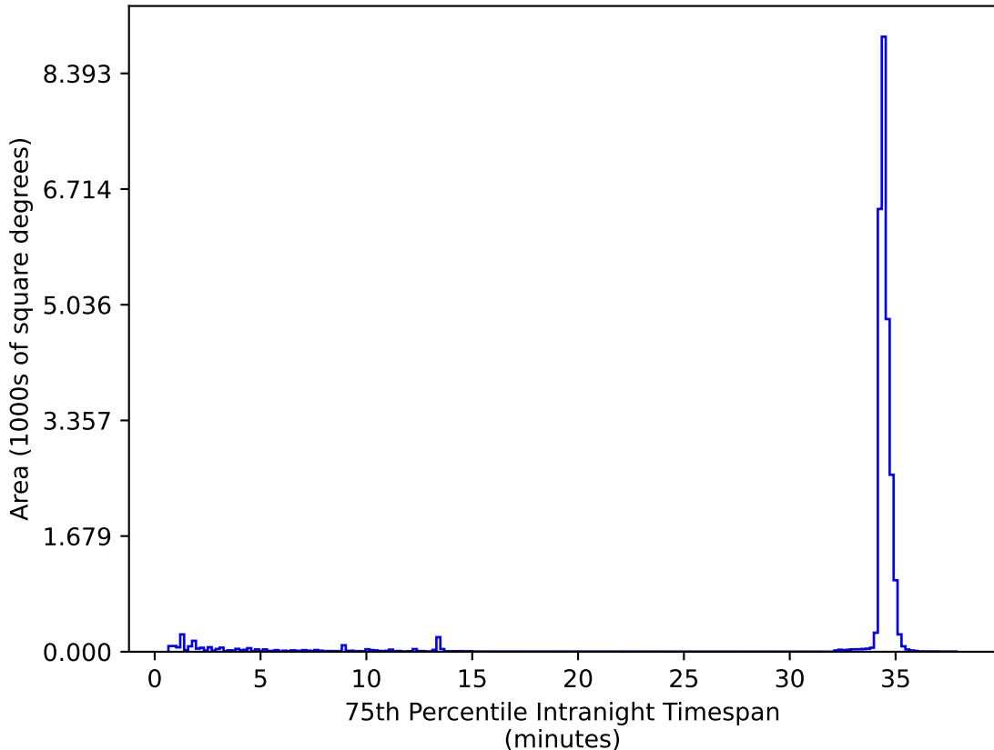
ddf_acor_sf10_lsf30_lsr10_v3.4_10yrs All sky zy bands: 75th Percentile Intranight Timespan
