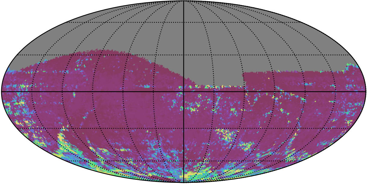
ddf_acor_sf10_lsf30_lsr10_v3.4_10yrs All sky z band: 75th Percentile Intranight Timespan
