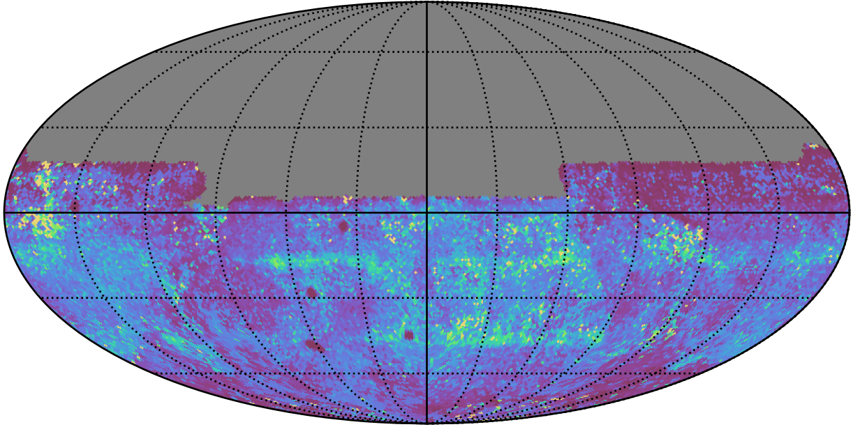
ddf_acor_sf10_lsf30_lsr10_v3.4_10yrs All sky y band: 75th Percentile Intranight Timespan
