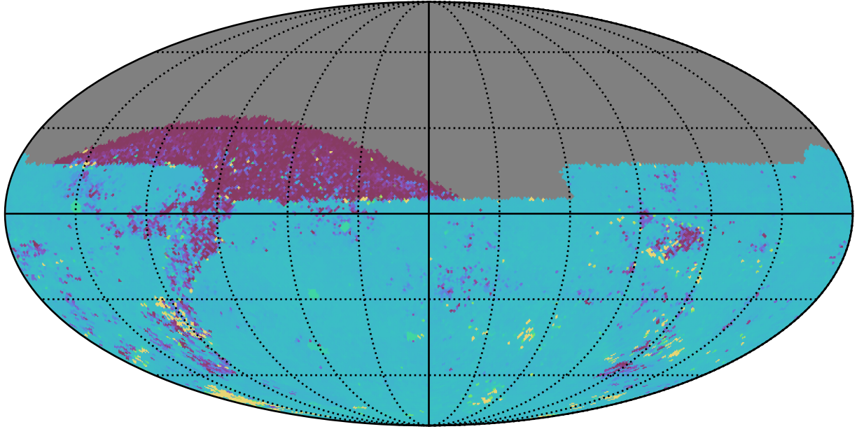
ddf_acor_sf10_lsf30_lsr10_v3.4_10yrs All sky ug bands: 75th Percentile Intranight Timespan
