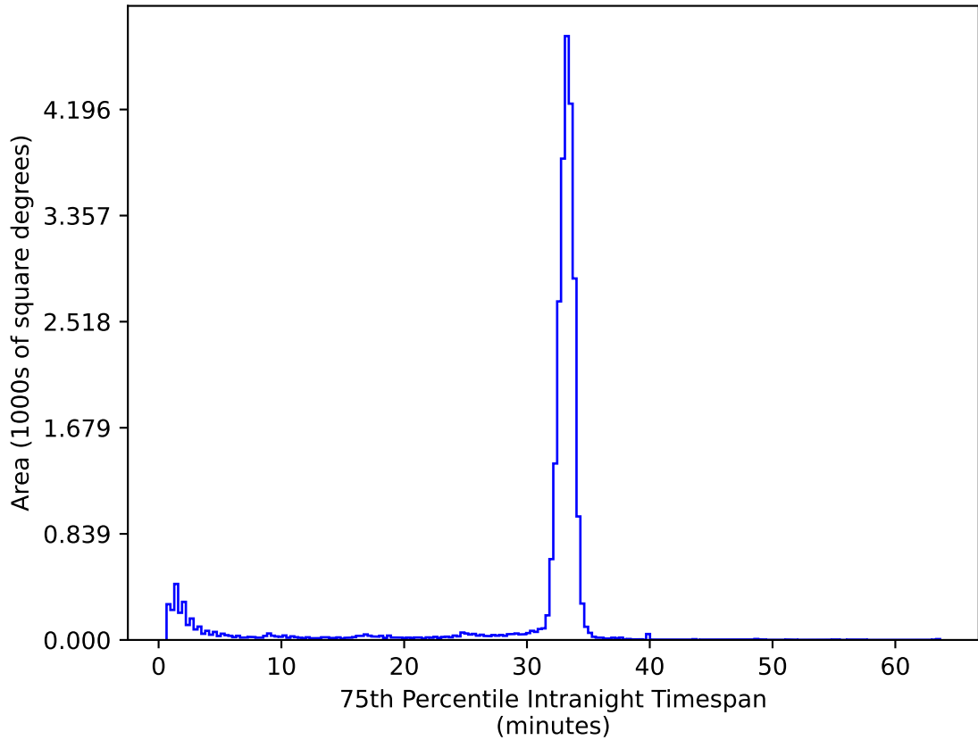
ddf_acor_sf10_lsf30_lsr10_v3.4_10yrs All sky ug bands: 75th Percentile Intranight Timespan
