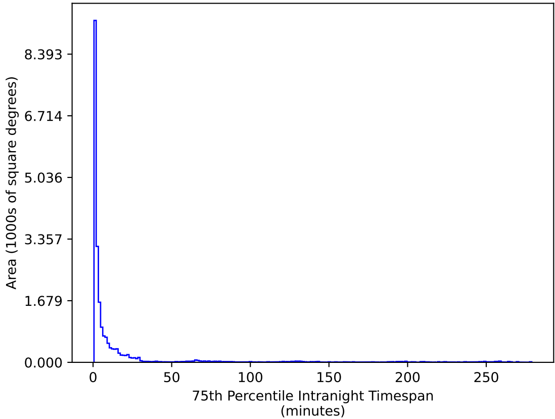
ddf_acor_sf10_lsf30_lsr10_v3.4_10yrs All sky u band: 75th Percentile Intranight Timespan
