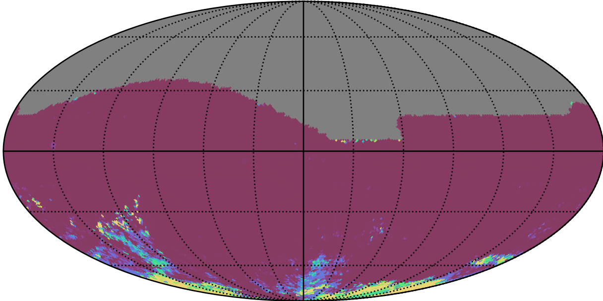
ddf_acor_sf10_lsf30_lsr10_v3.4_10yrs All sky ri bands: 75th Percentile Intranight Timespan
