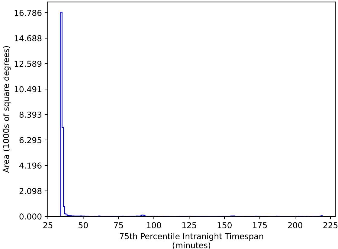
ddf_acor_sf10_lsf30_lsr10_v3.4_10yrs All sky ri bands: 75th Percentile Intranight Timespan
