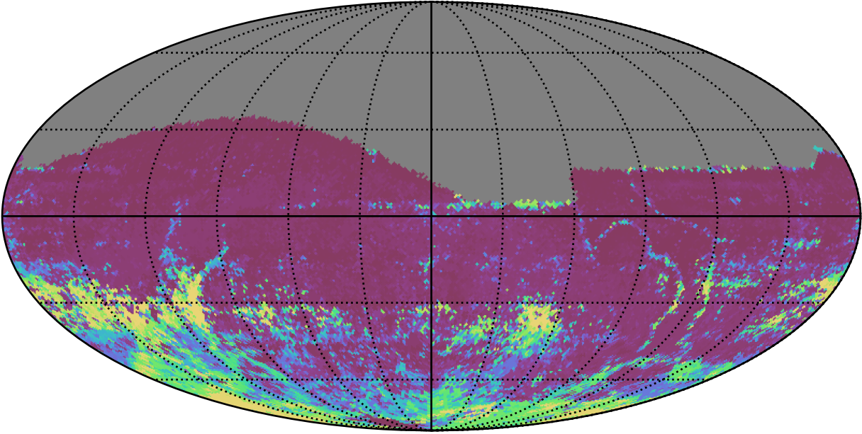
ddf_acor_sf10_lsf30_lsr10_v3.4_10yrs All sky r band: 75th Percentile Intranight Timespan
