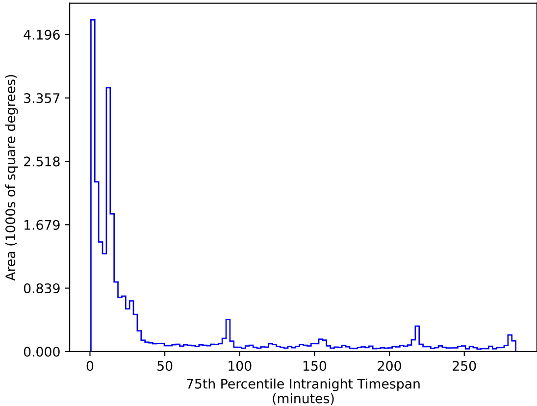
ddf_acor_sf10_lsf30_lsr10_v3.4_10yrs All sky r band: 75th Percentile Intranight Timespan
