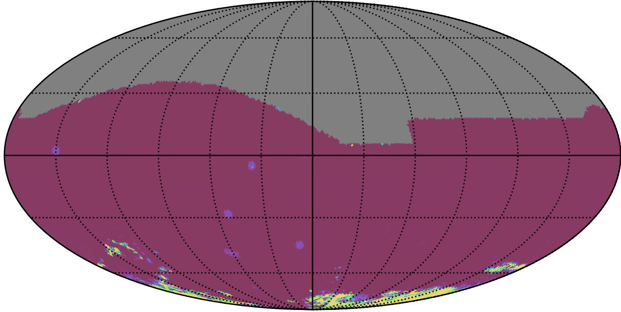
ddf_acor_sf10_lsf30_lsr10_v3.4_10yrs All sky iz bands: 75th Percentile Intranight Timespan
