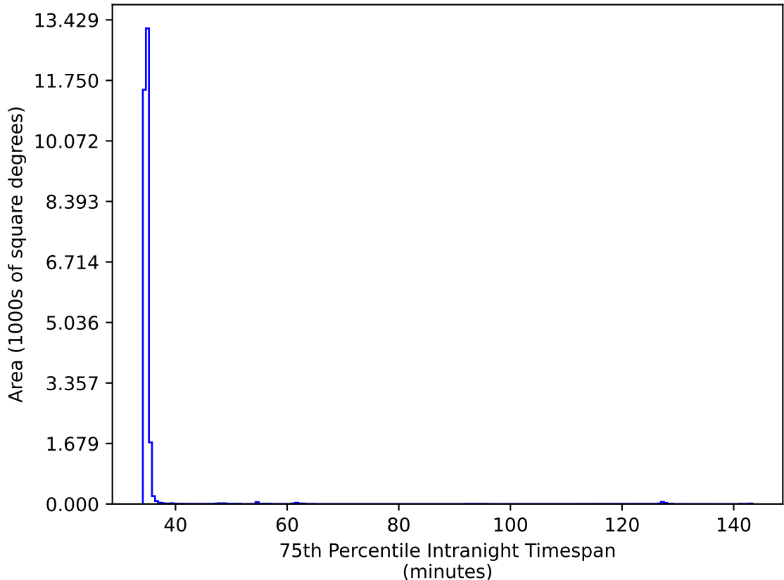
ddf_acor_sf10_lsf30_lsr10_v3.4_10yrs All sky iz bands: 75th Percentile Intranight Timespan
