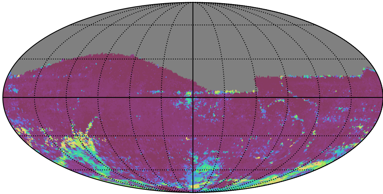
ddf_acor_sf10_lsf30_lsr10_v3.4_10yrs All sky i band: 75th Percentile Intranight Timespan
