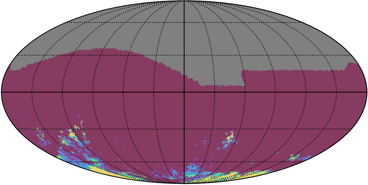
ddf_acor_sf10_lsf30_lsr10_v3.4_10yrs All sky gr bands: 75th Percentile Intranight Timespan
