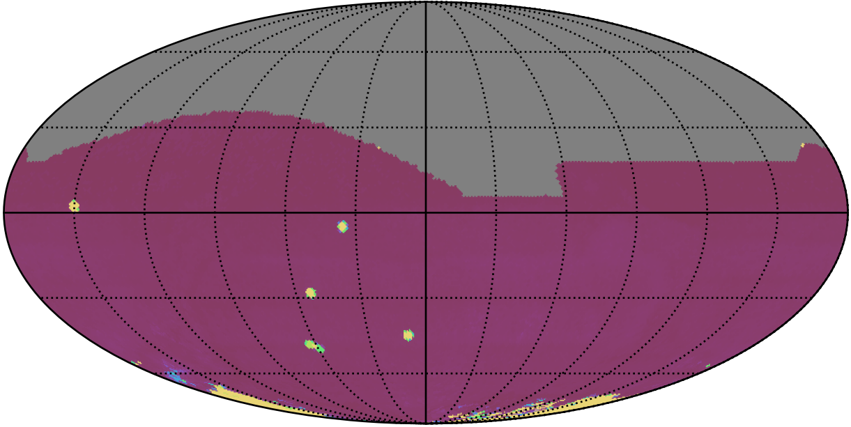
ddf_acor_sf10_lsf30_lsr10_v3.4_10yrs All sky all bands: 75th Percentile Intranight Timespan
