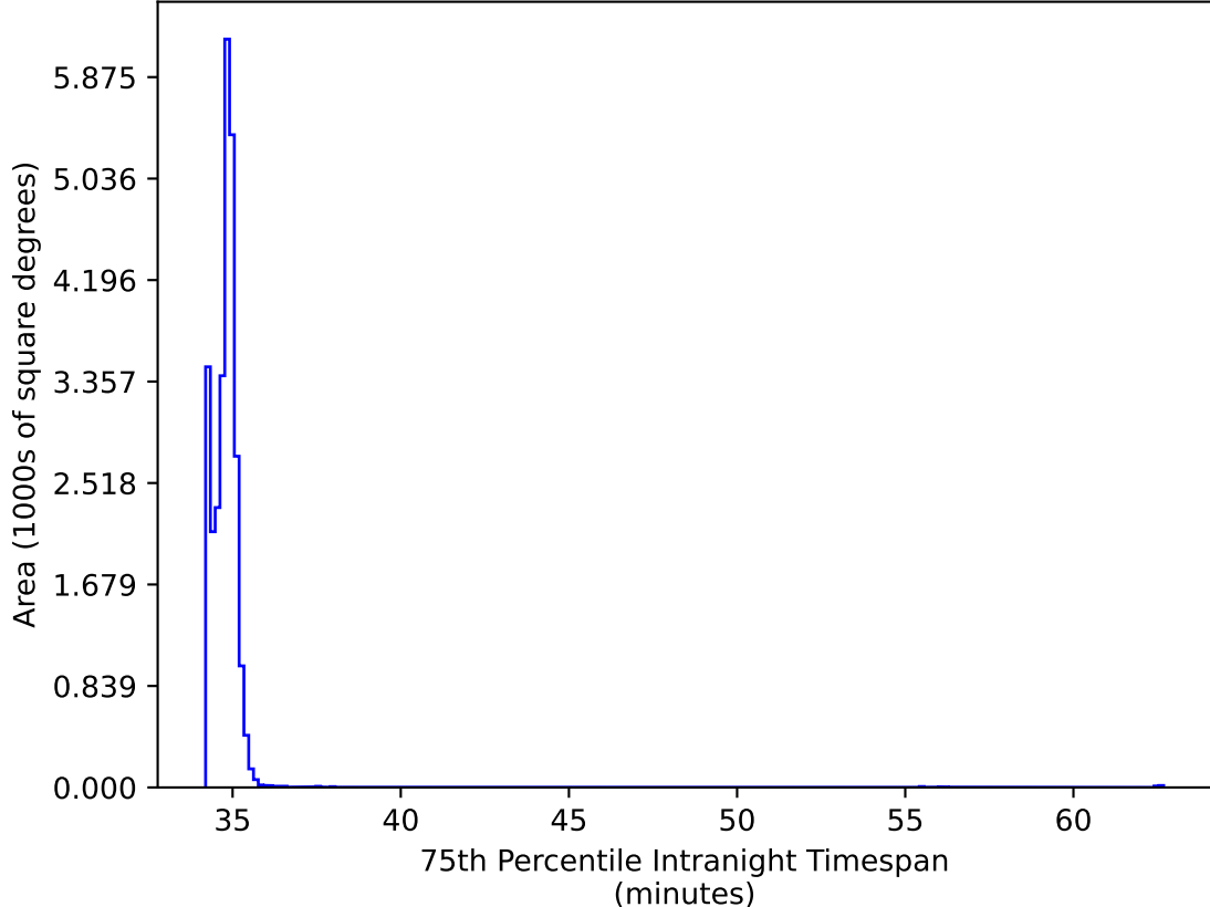
ddf_acor_sf10_lsf30_lsr10_v3.4_10yrs All sky all bands: 75th Percentile Intranight Timespan
