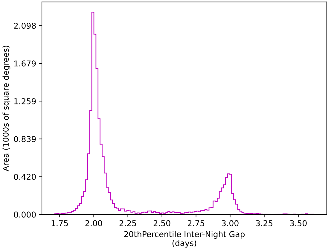
ddf_acor_sf10_lsf30_lsr10_v3.4_10yrs WFD z band: 20thPercentile Inter-Night Gap
