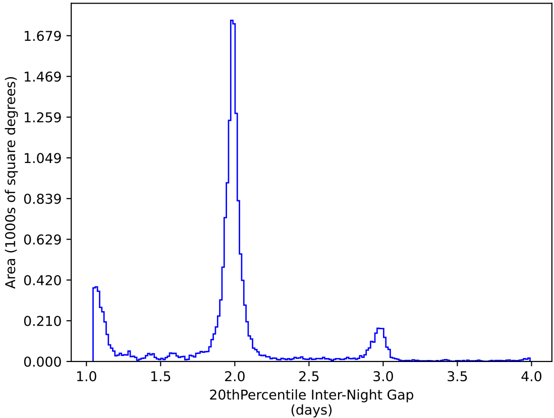
ddf_acor_sf10_lsf30_lsr10_v3.4_10yrs WFD y band: 20thPercentile Inter-Night Gap
