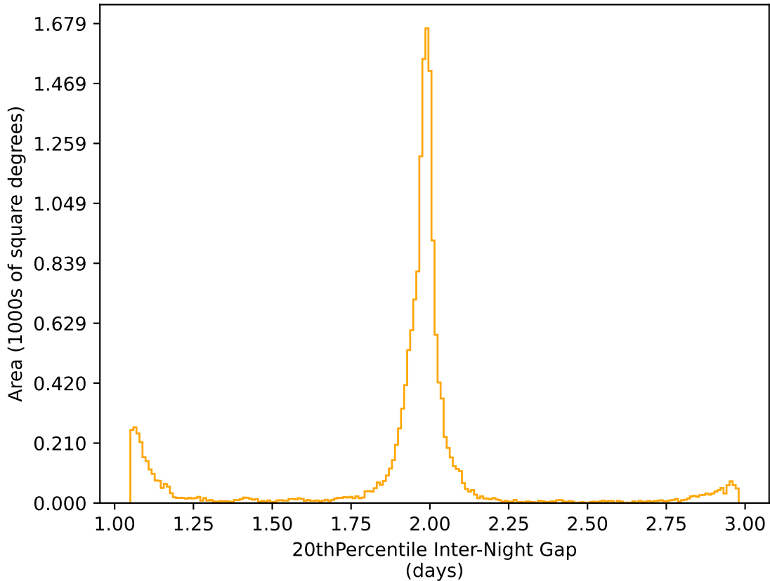
ddf_acor_sf10_lsf30_lsr10_v3.4_10yrs WFD r band: 20thPercentile Inter-Night Gap
