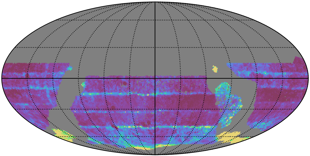
ddf_acor_sf10_lsf30_lsr10_v3.4_10yrs WFD all bands: 20thPercentile Inter-Night Gap
