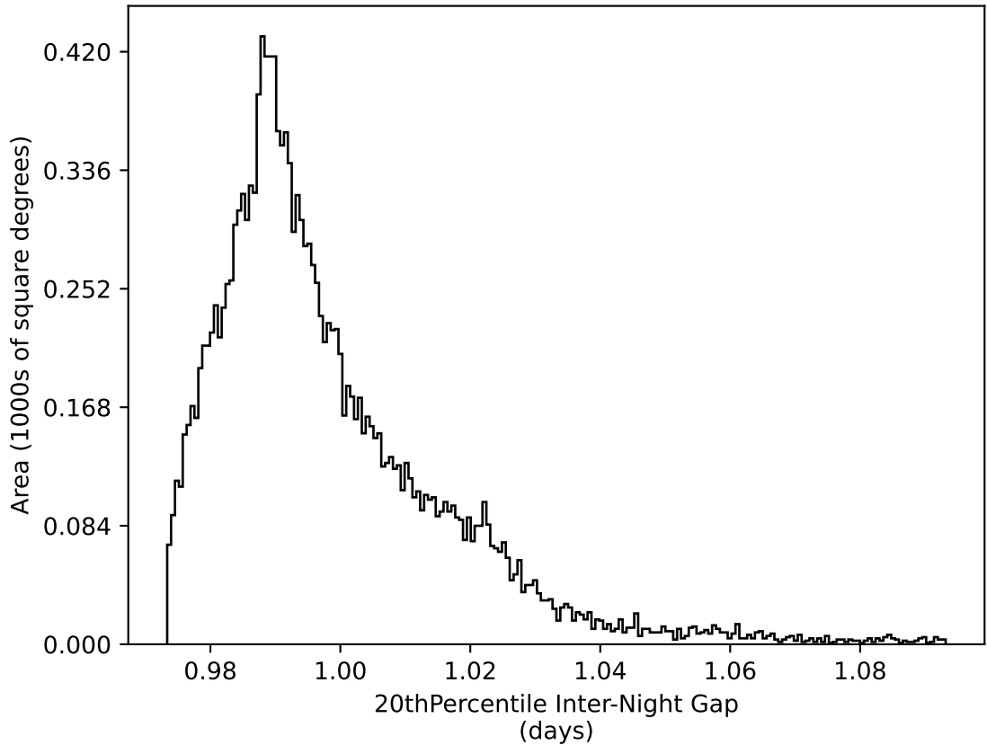
ddf_acor_sf10_ls30_lsr10_v3.4_10yrs WFD all bands: 20thPercentile Inter-Night Gap
