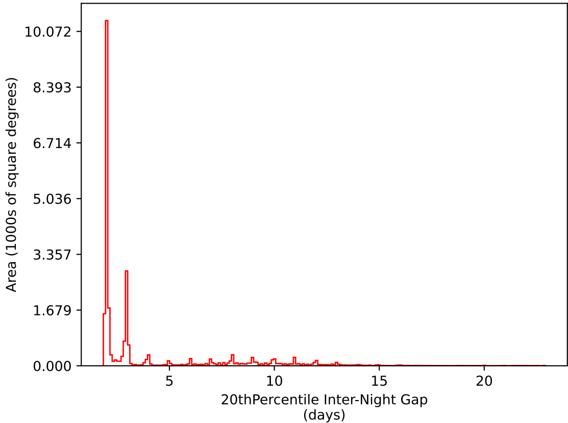
ddf_acor_sf10_lsf30_lsr10_v3.4_10yrs All sky i band: 20thPercentile Inter-Night Gap
