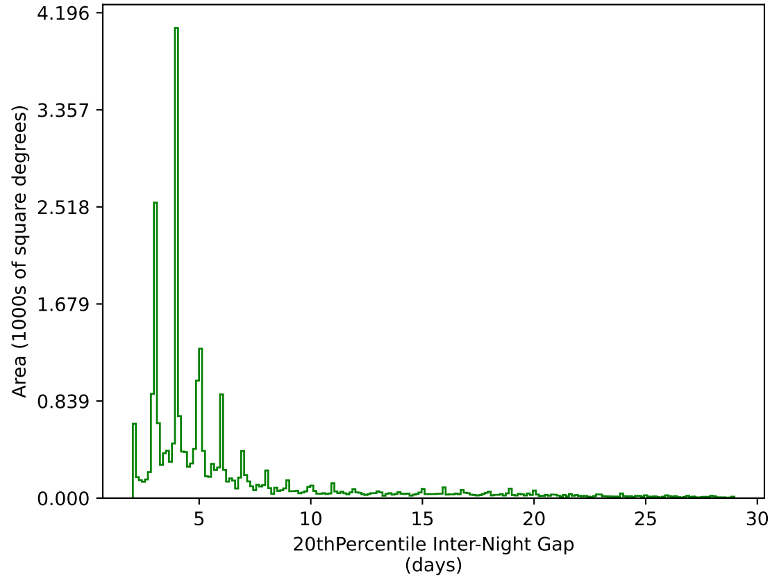
ddf_acor_sf10_ls30_lsr10_v3.4_10yrs All sky g band: 20thPercentile Inter-Night Gap
