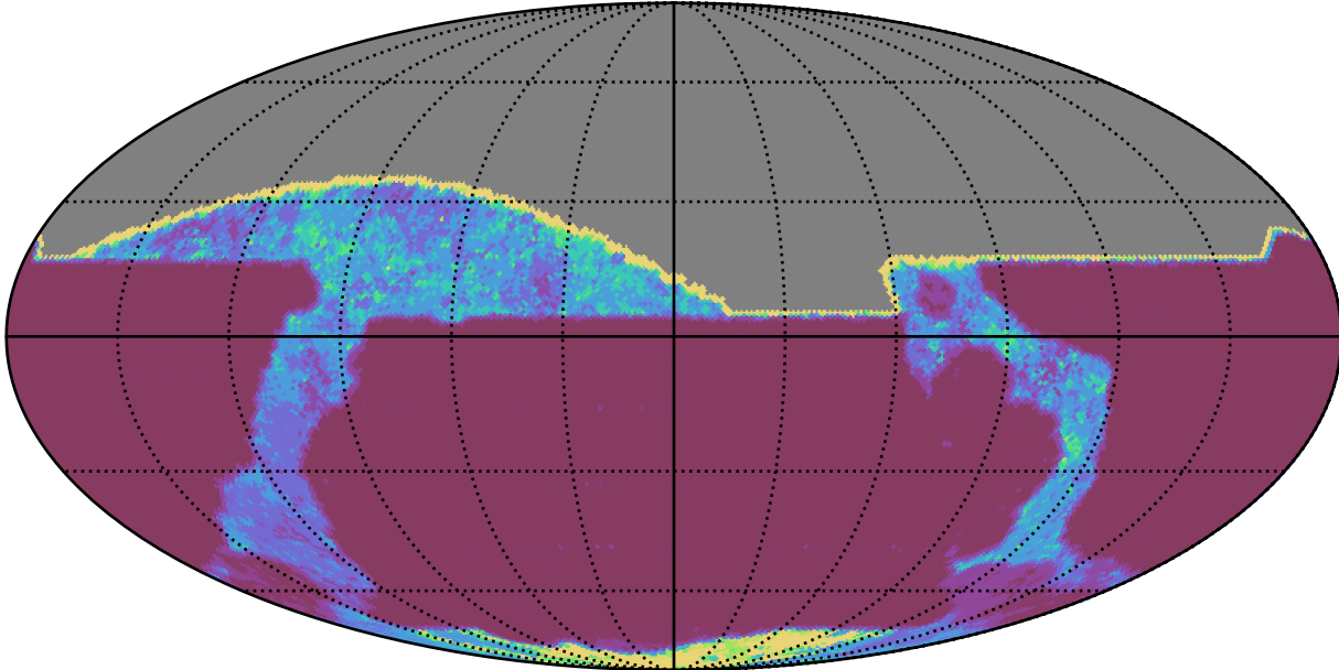
ddf_acor_sf10_lsf30_lsr10_v3.4_10yrs All sky all bands: 20thPercentile Inter-Night Gap
