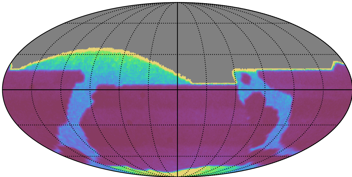
ddf_acor_sf10_lsf30_lsr10_v3.4_10yrs : properMotion
