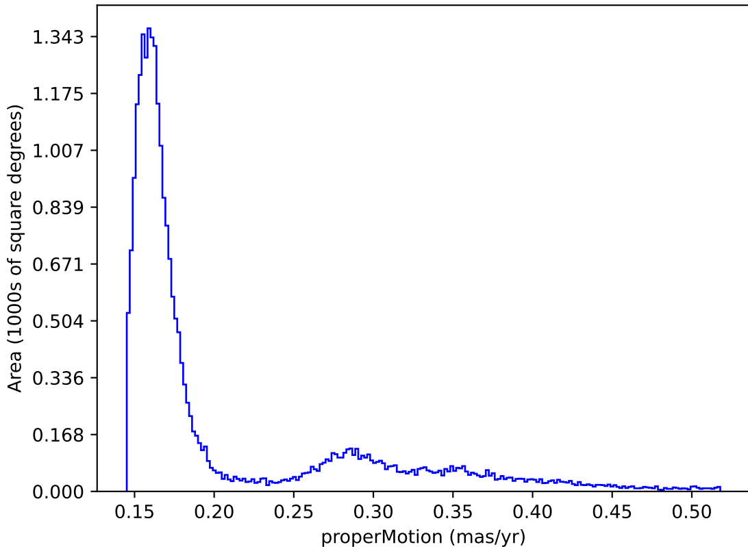
ddf_acor_sf10_ls30_lsr10_v3.4_10yrs : properMotion
