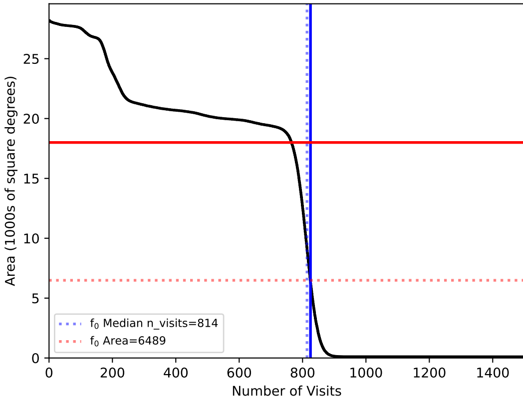
ddf_acor_sf10_lsf30_lsr10_v3.4_10yrs : fO
