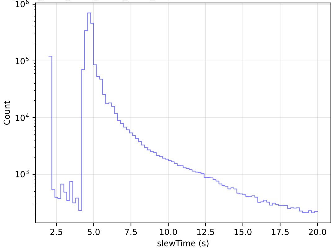
ddf_acor_sf10_lsf30_lsr10_v3.4_10yrs All visits: Zoom Slew Time Histogram
