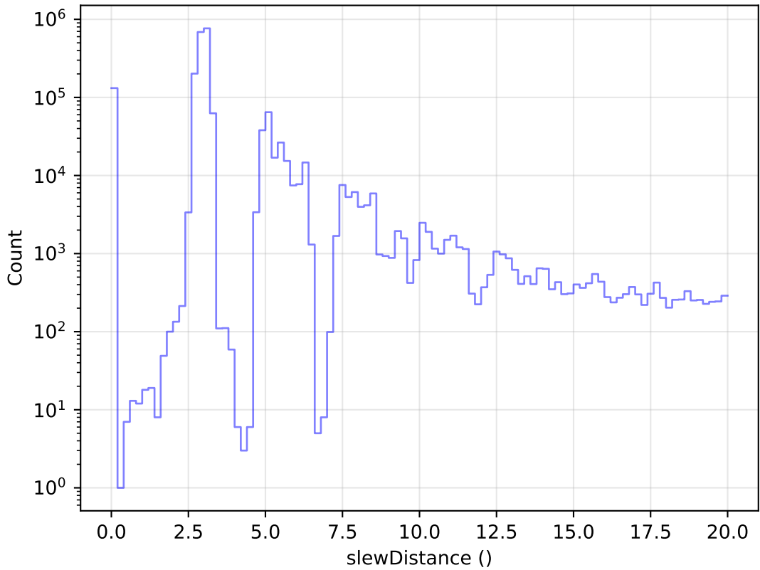
ddf_acor_sf10_lsf30_lsr10_v3.4_10yrs All visits: Zoom Slew Distance Histogram
