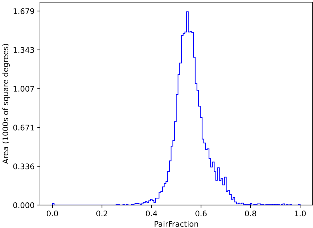
ddf_acor_sf10_lsf30_lsr10_v3.4_10yrs (g or r or i): PairFraction
