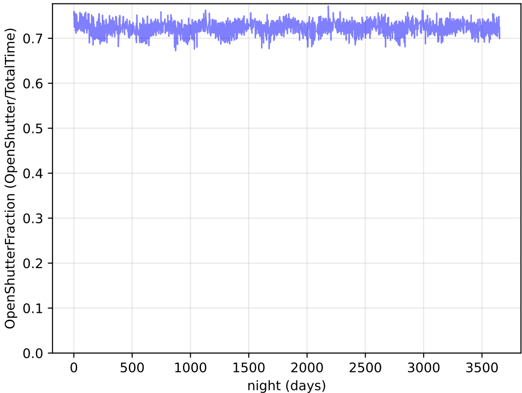
ddf_acor_sf10_lsf30_lsr10_v3.4_10yrs : OpenShutterFraction
