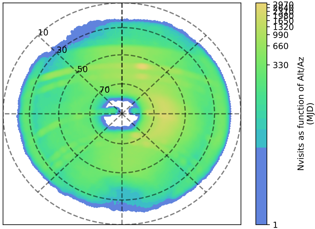
ddf_acor_sf10_lsf30_lsr10_v3.4_10yrs z: Nvisits as function of Alt/Az
