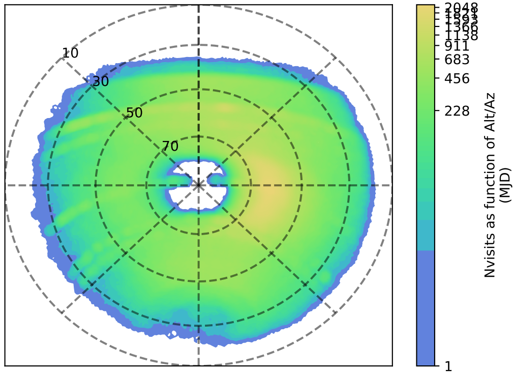
ddf_acor_sf10_lsf30_lsr10_v3.4_10yrs y: Nvisits as function of Alt/Az
