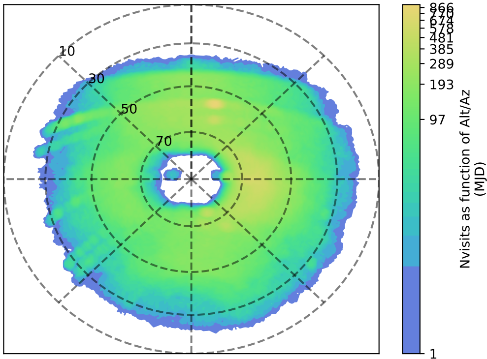
ddf_acor_sf10_ls30_lsr10_v3.4_10yrs u: Nvisits as function of Alt/Az
